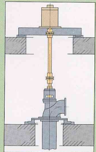
Two-floor installation
